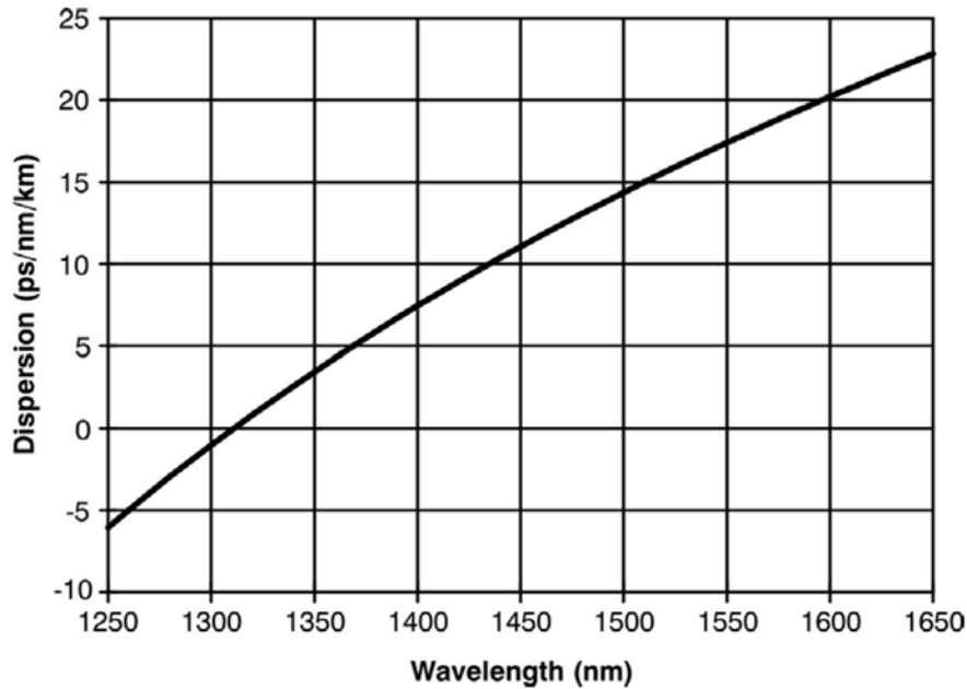
Figure 1 - Dispersion Characteristics of NDSF
