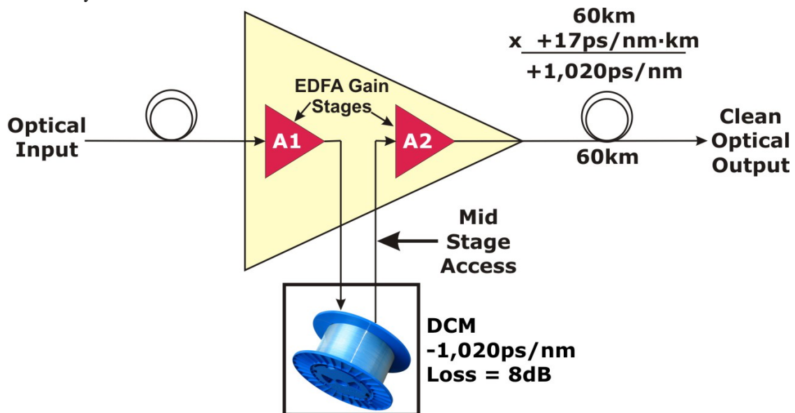
Figure 3 - Typical DCM Application
