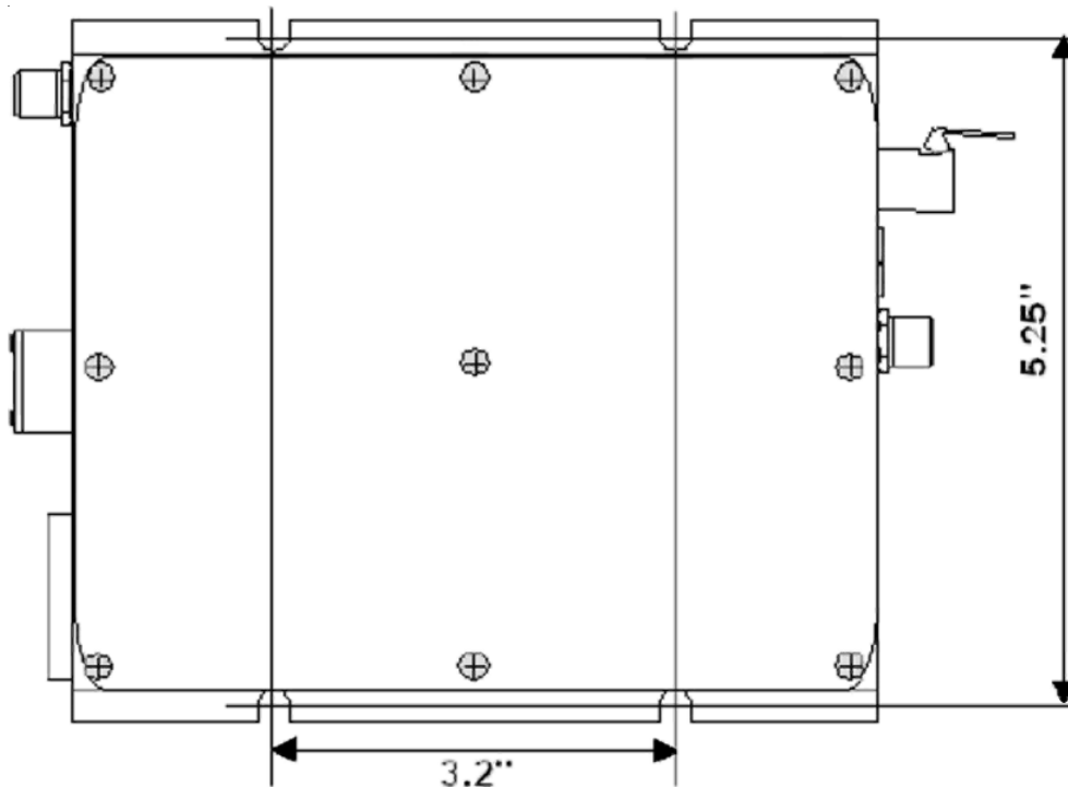
FIGURE 1 - OTOT-1000-FF MOUNTING DIAGRAM
