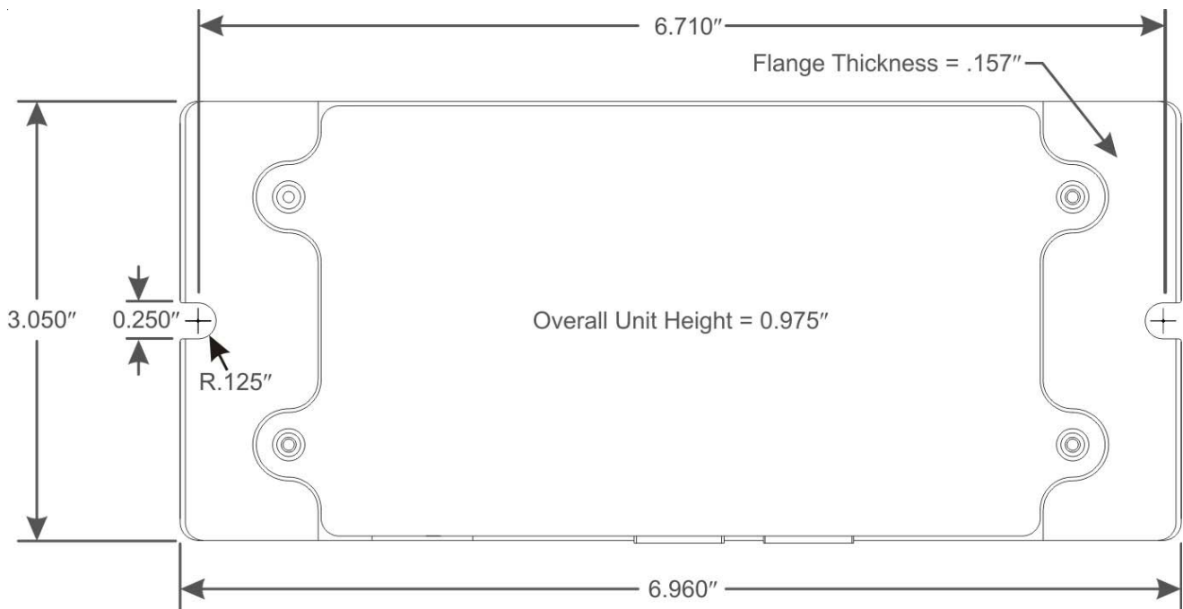
OTPN-400C Key Dimensions
