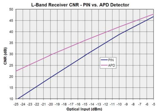
Adv. L-Band Rx CNR with PIN & APD
